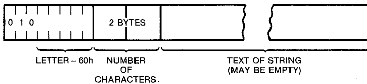
Fig. 3-6. Data structure for string variable.
